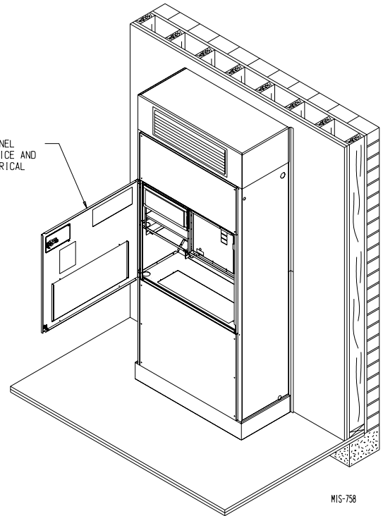
Unit installed with free blow plenum box
