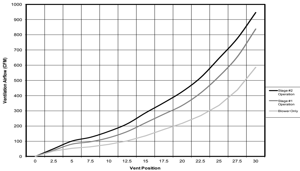
CRVMP-5 WA5S/WL5S Ventilation Airflow
