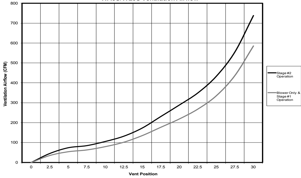
CRVMP-5 WA4S/WL4S Ventilation Airflow
