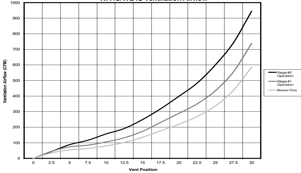
CRVMP-5 WA4S/WL4S Ventilation Airflow
