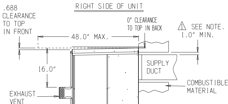
FIGURE 1 COMBUSTIBLE CLEARANCE
