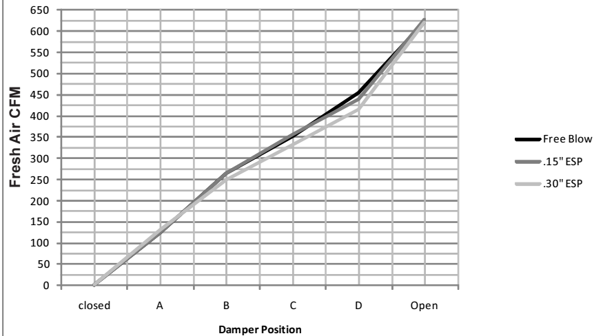
W30-36G CRV Airflow Versus Position - Low Speed
